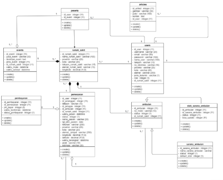
Gambar 3 Class Diagram
